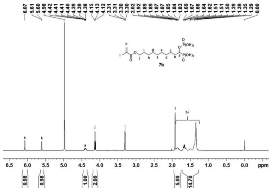
Figure 10: ^1\text{H-NMR} spectrum of monomer 7b [16].
